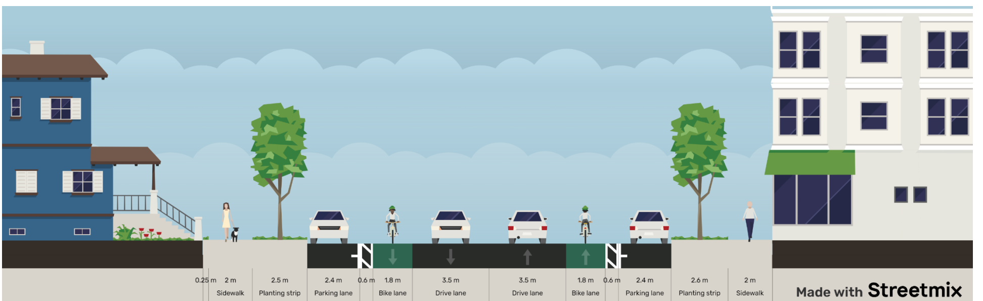
Figure 9 Collector (26 m Right-of-Way) On-Street Parking (Both-Sides) with Bike Lanes
