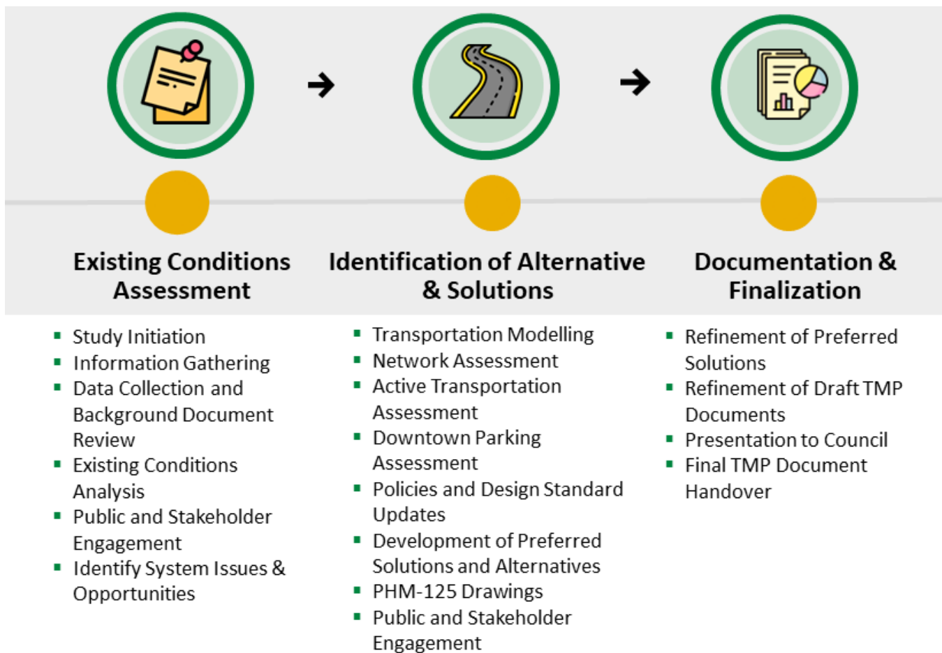
Figure 2 Project Methodology
