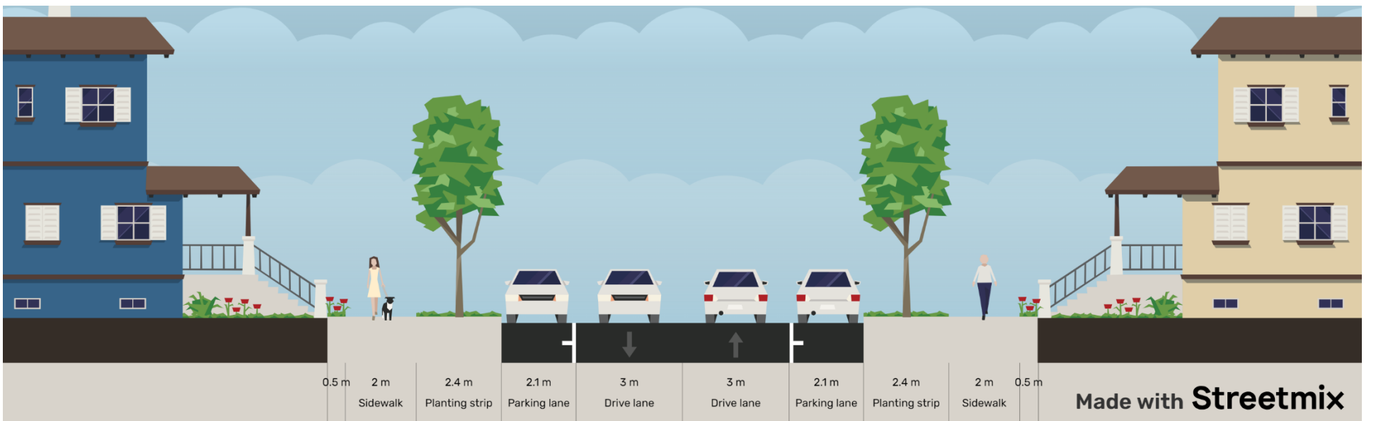
Figure 7 Local Road (20 m Right-of-Way) On-Street Parking (Both-Sides)
