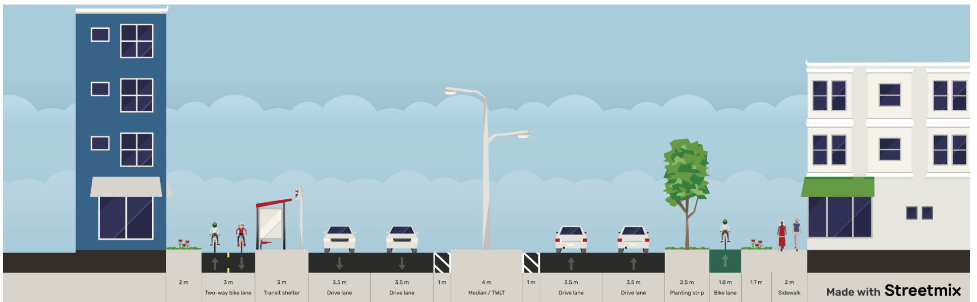
Figure 11 Arterial (36 m Right-of-Way) with Median / TWLTL
